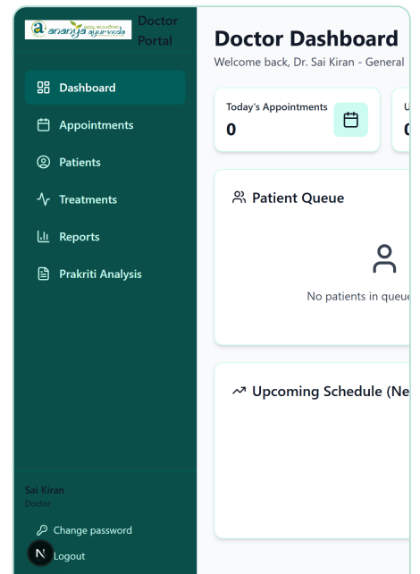
Doctor workflow
